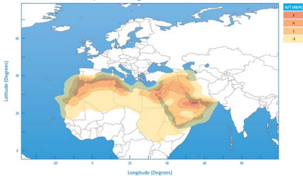
Es'hail-1 Ka-Band uplink coverage over MENA
